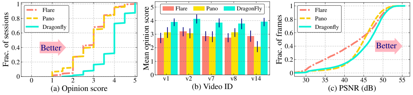
Figure 14: Results from user study. (a) Distribution of opinion scores across all users and sessions; (b) MOS per video along with 95% confidence intervals. Video IDs correspond to naming in [34]; and (c) Distribution of PSNR across users and sessions.
